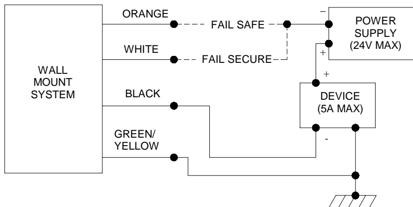
Wall Mount System Wiring Diagram 2
