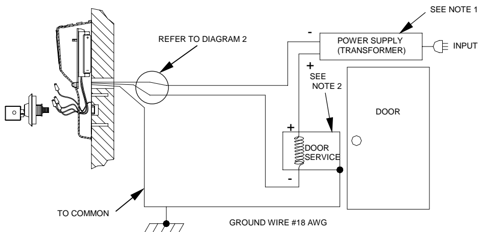
(EXAMPLE) Wall Mount System Wiring Diagram 1
